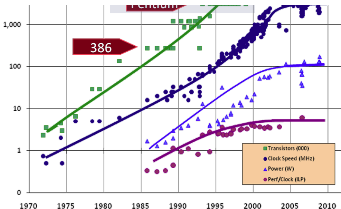
Figure 1: Intel CPU Introductions (graph updated August 2009; article text original from December 2004)
