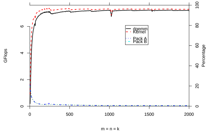
Fig. 18. POWER5 (1.9 MHz).
